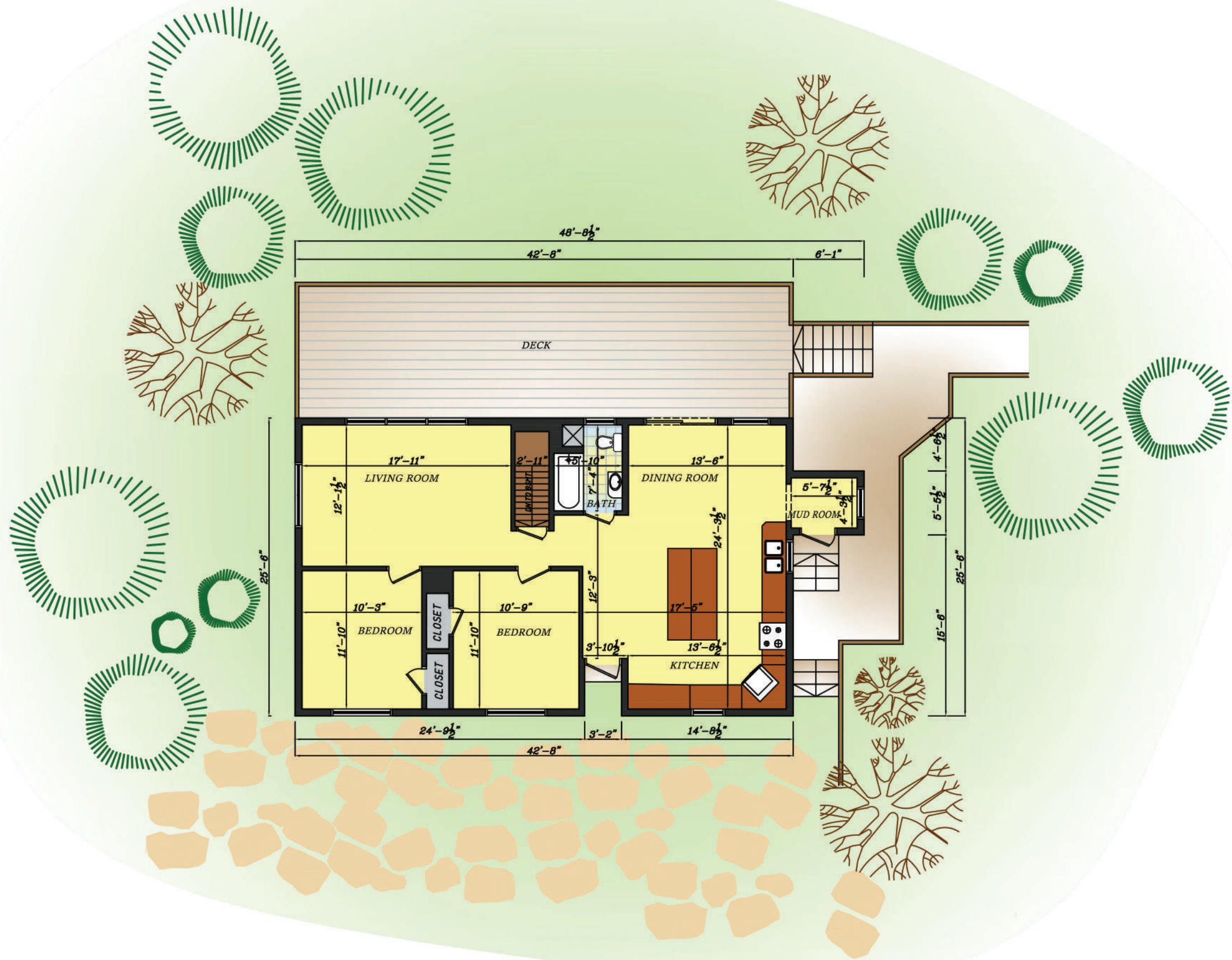
Main Level Floor Plan 58 Shore Road Lunenburg, NS
